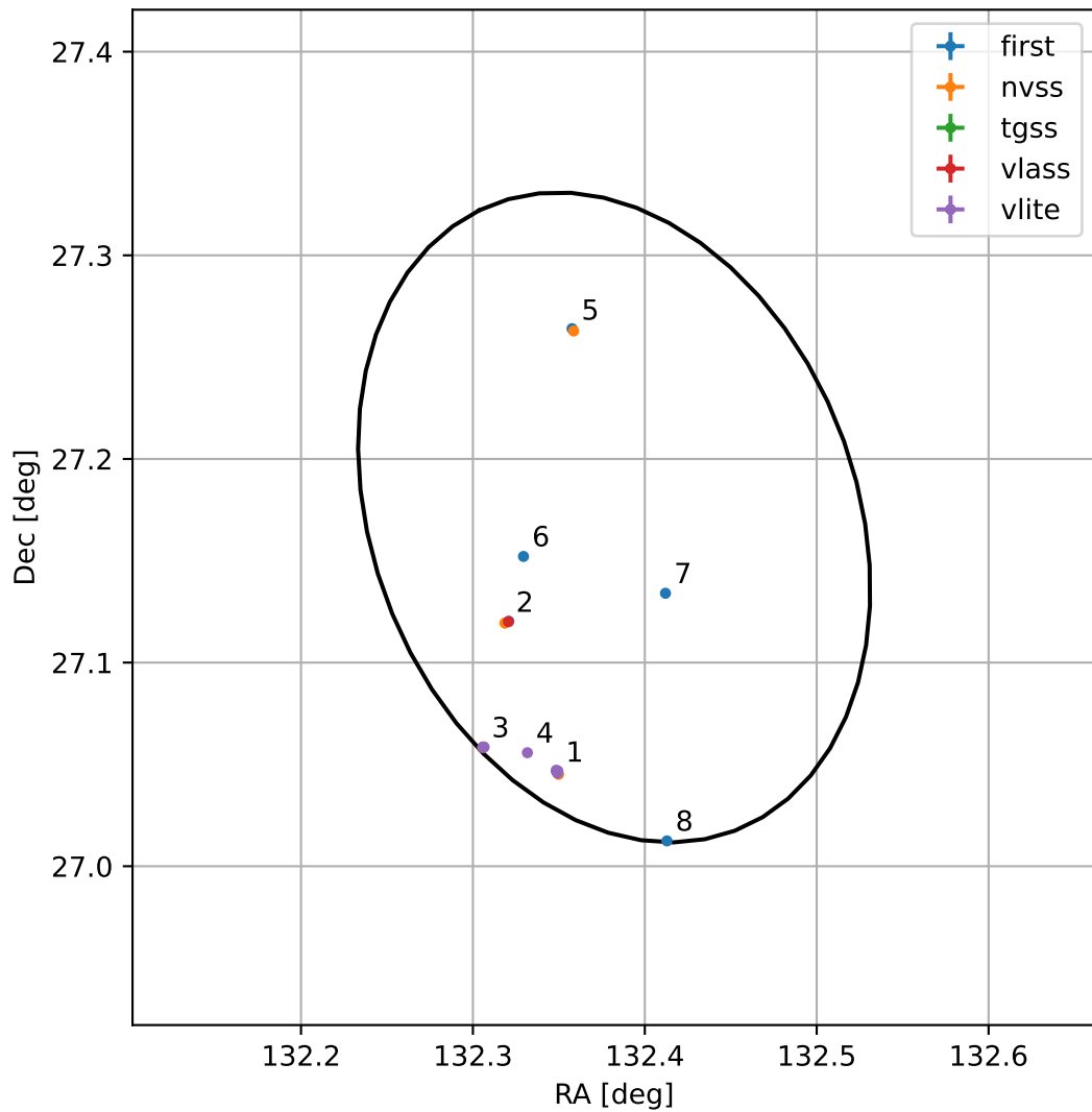
4FGL J0849.5+2710
