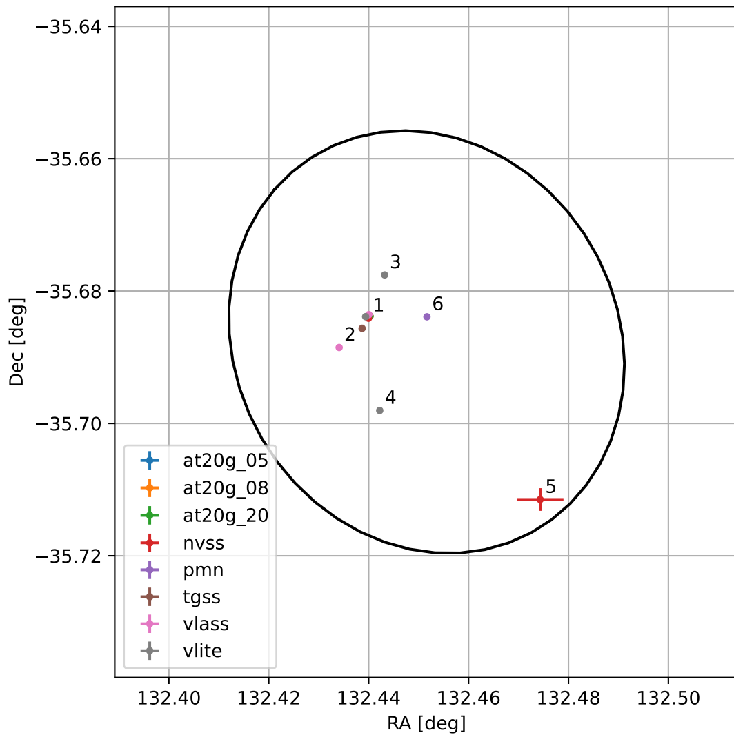
4FGL J0849.8-3541
