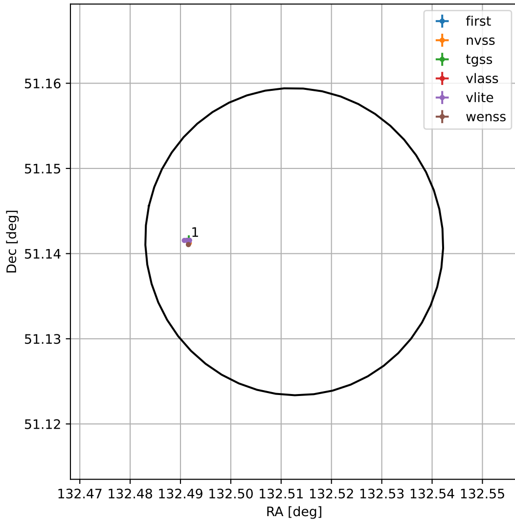
4FGL J0850.0+5108
