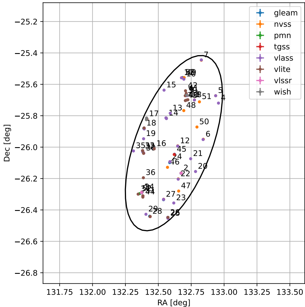
4FGL J0850.4-2558
