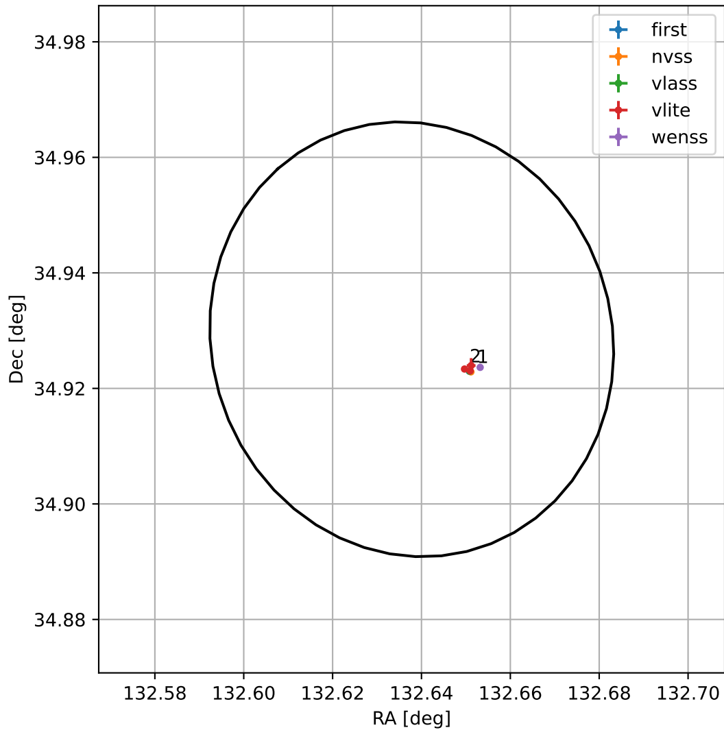
4FGL J0850.5+3455
