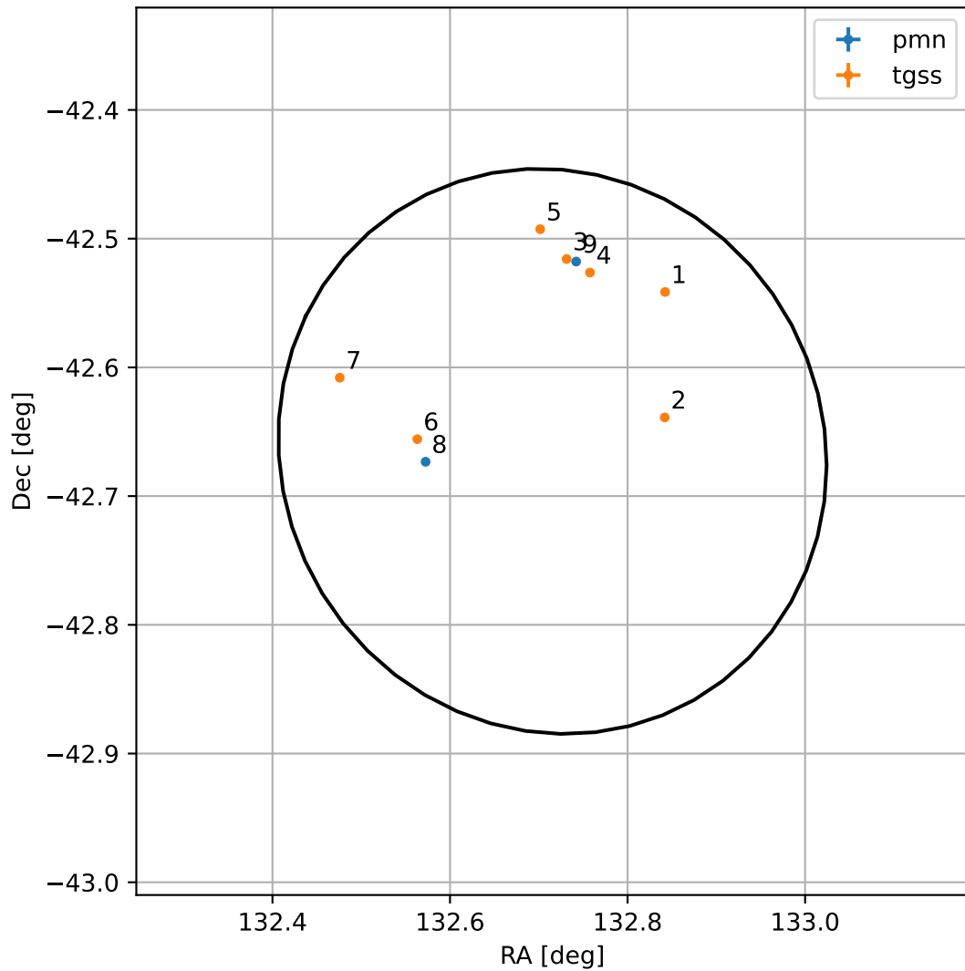
4FGL J0850.8-4239
