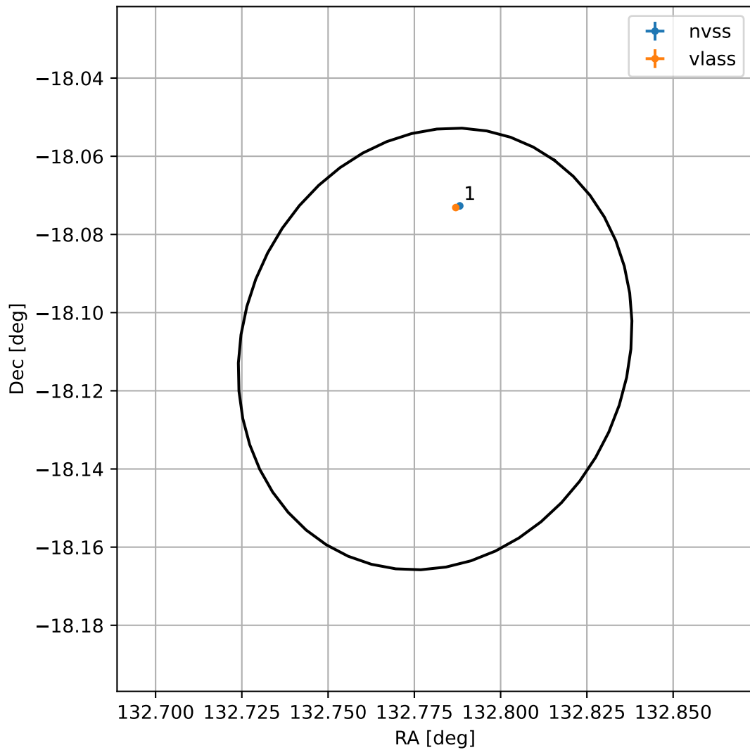
4FGL J0851.1-1806
