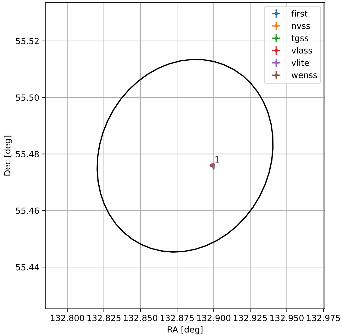
4FGL J0851.5+5528
