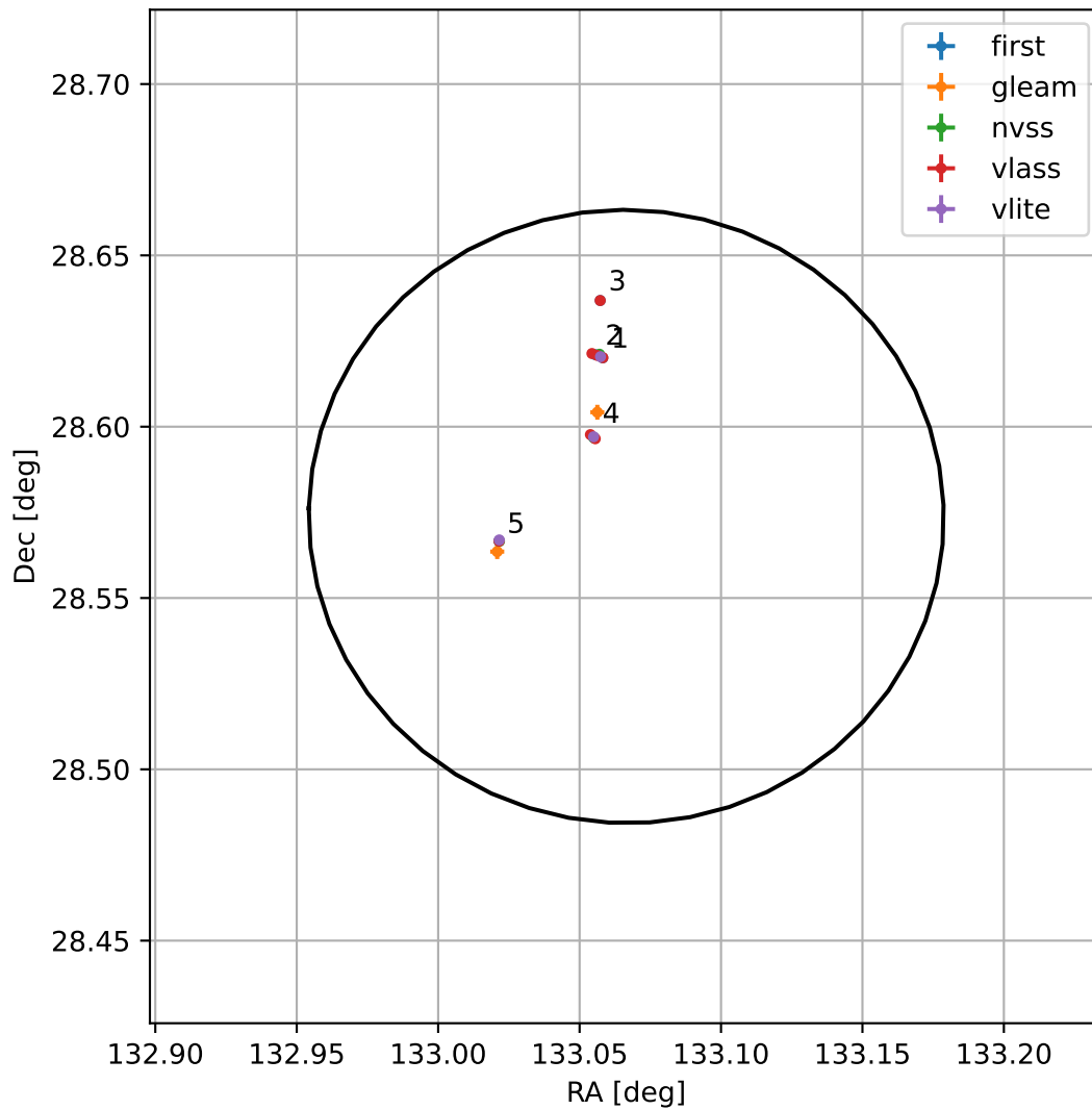
4FGL J0852.2+2834
