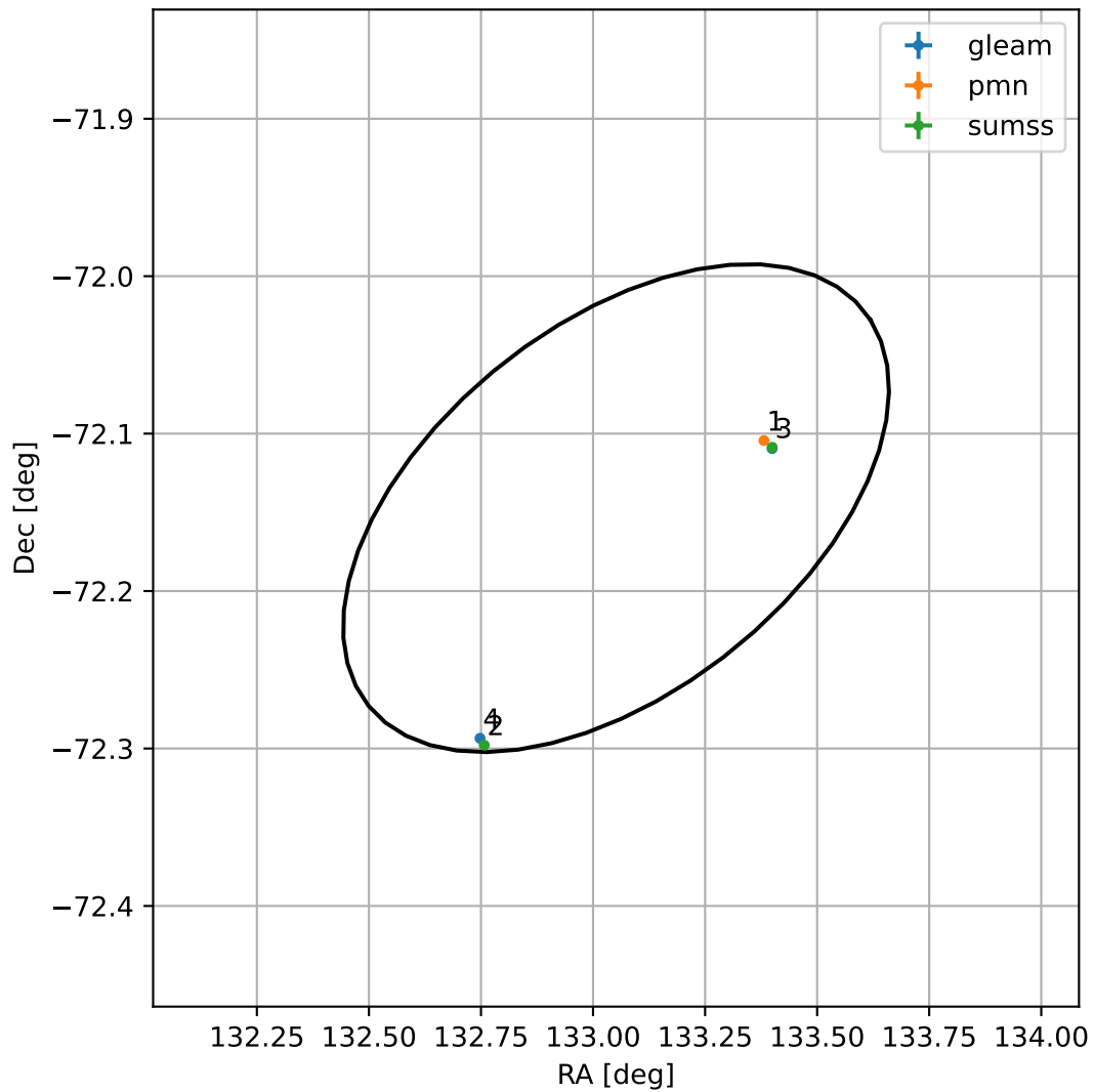
4FGL J0852.2-7208
