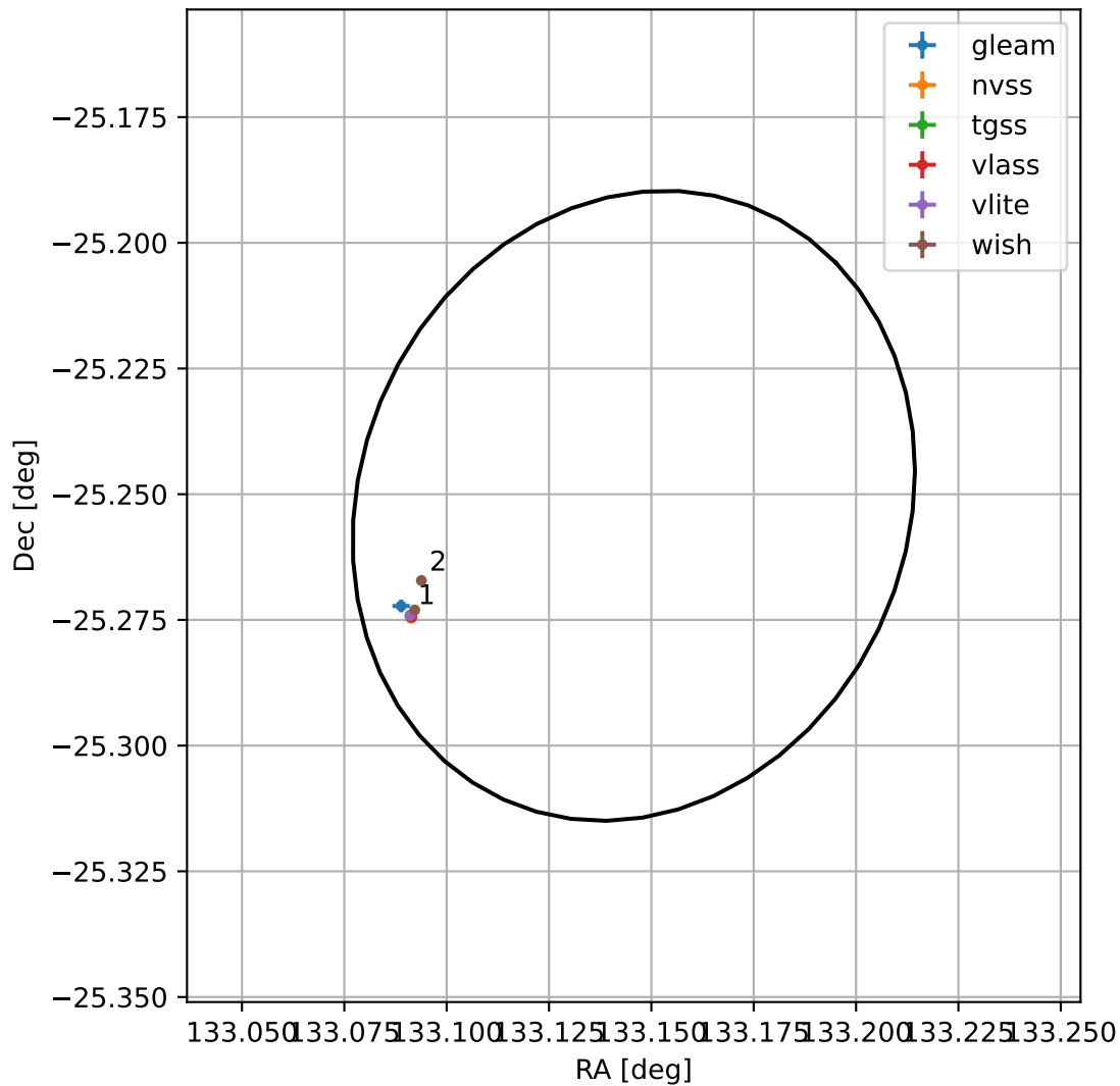
4FGL J0852.5-2515
