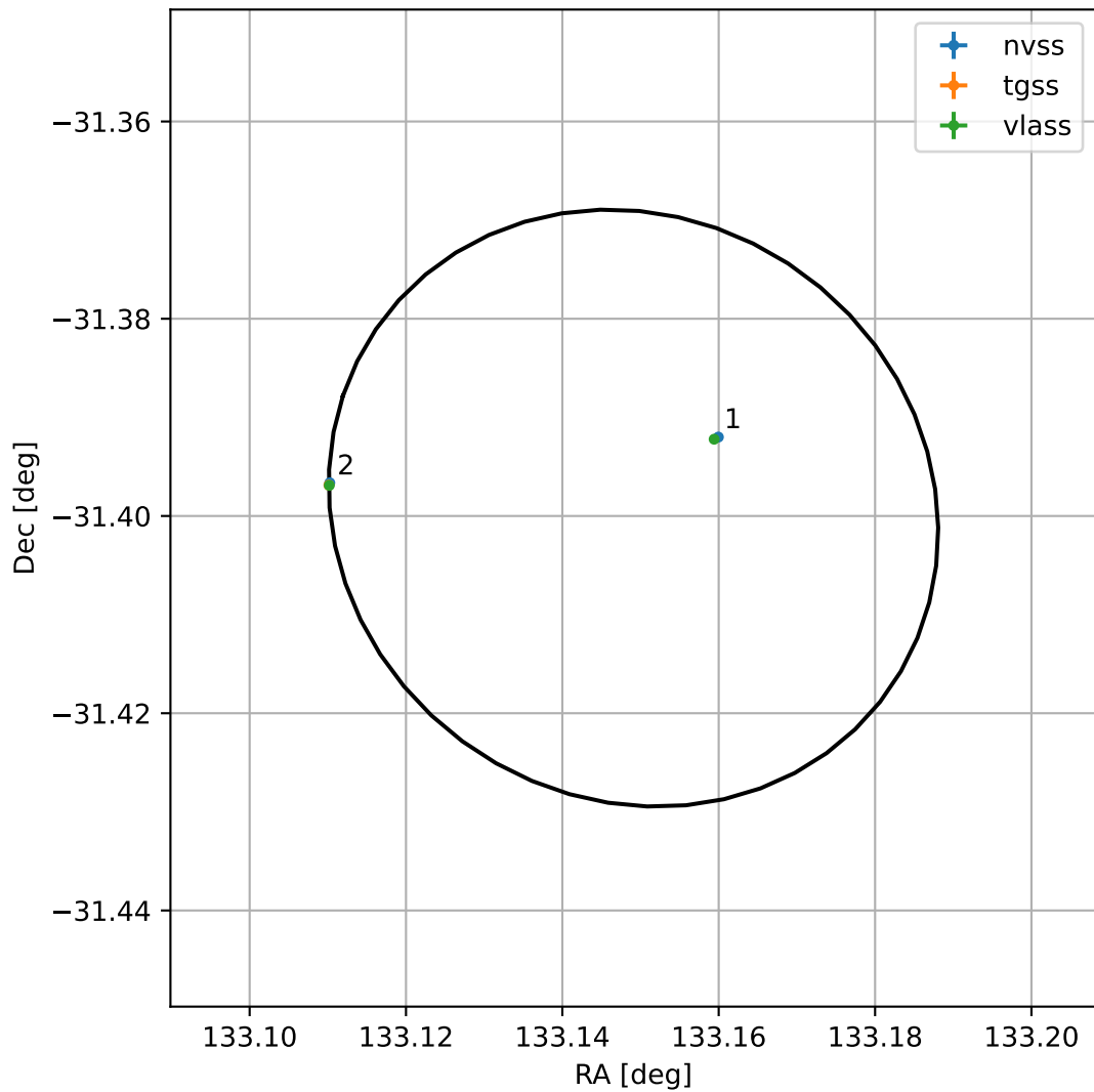
4FGL J0852.5-3123
