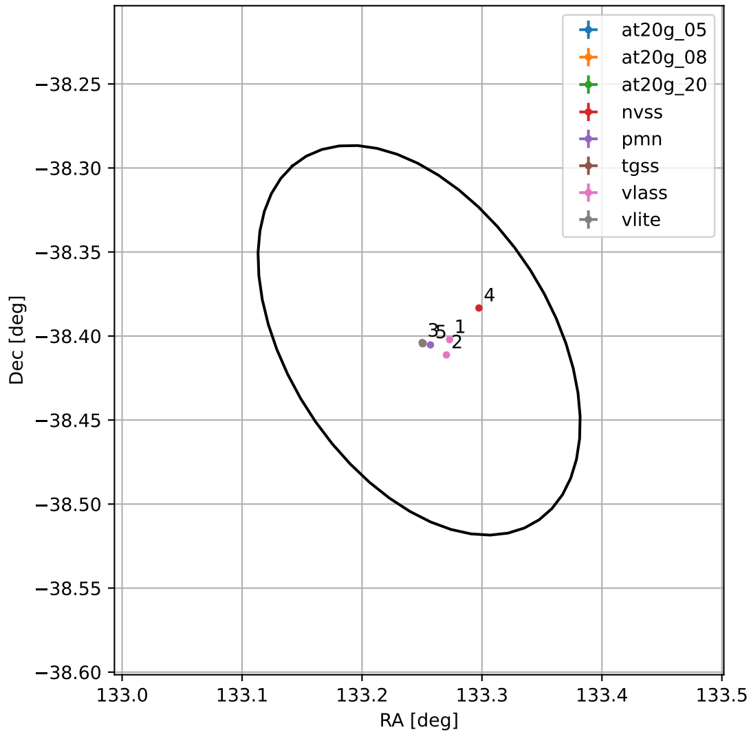
4FGL J0852.9-3824
