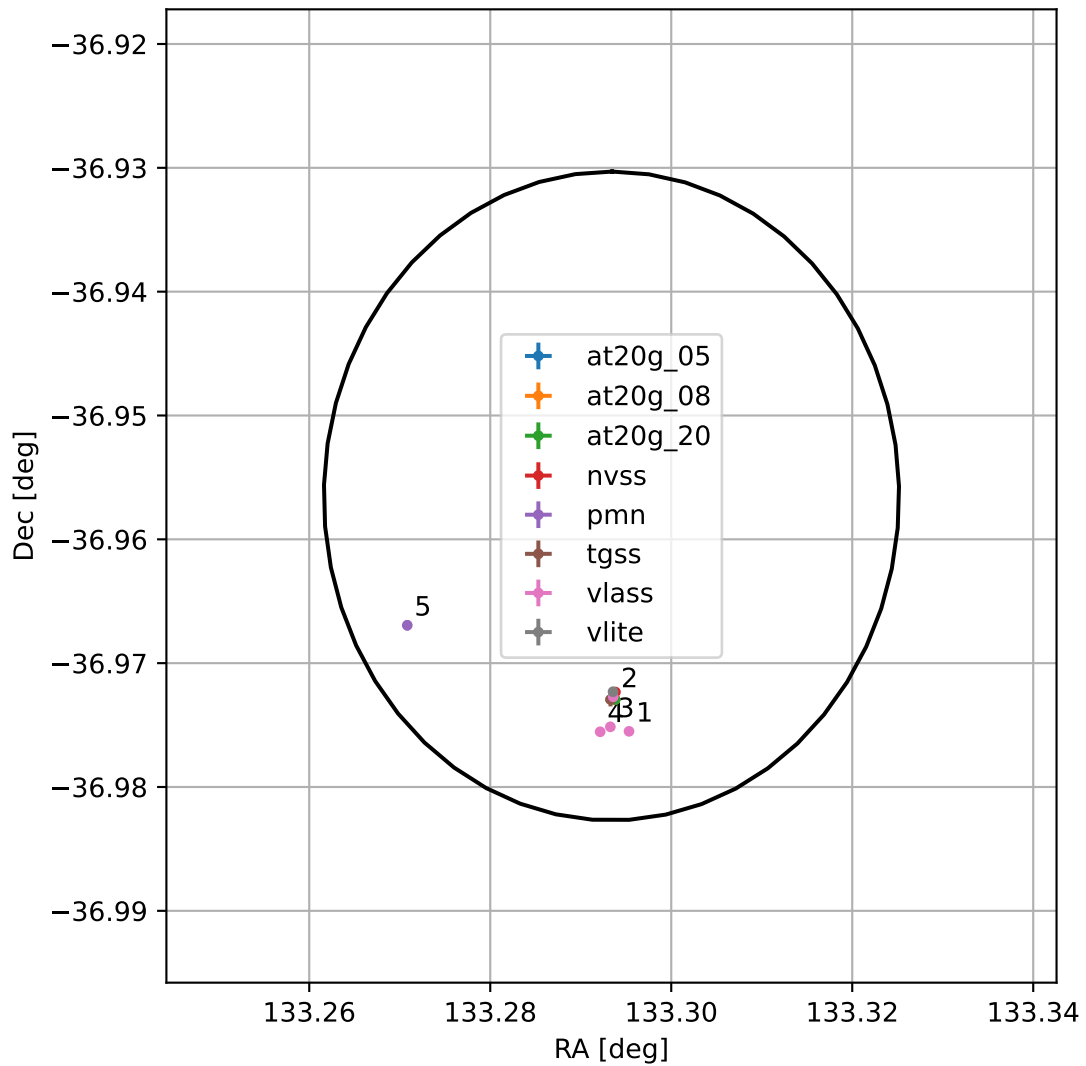
4FGL J0853.1-3657
