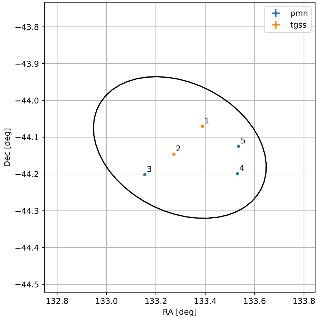
4FGL J0853.1-4407
