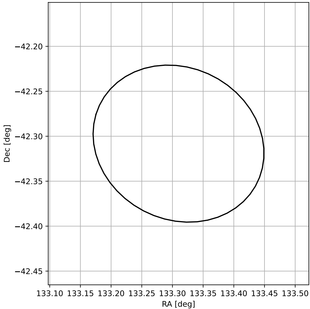
4FGL J0853.2-4218
