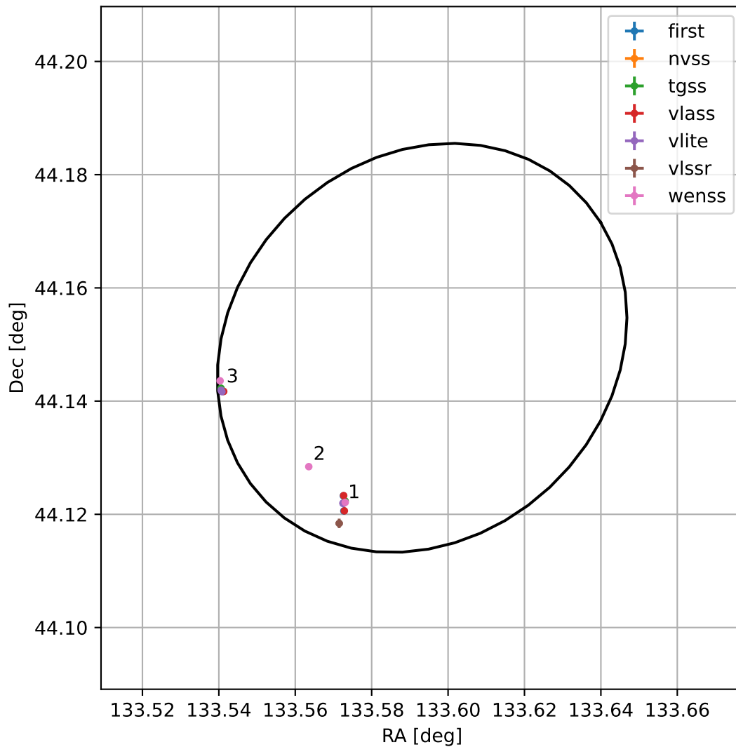
4FGL J0854.3+4408
