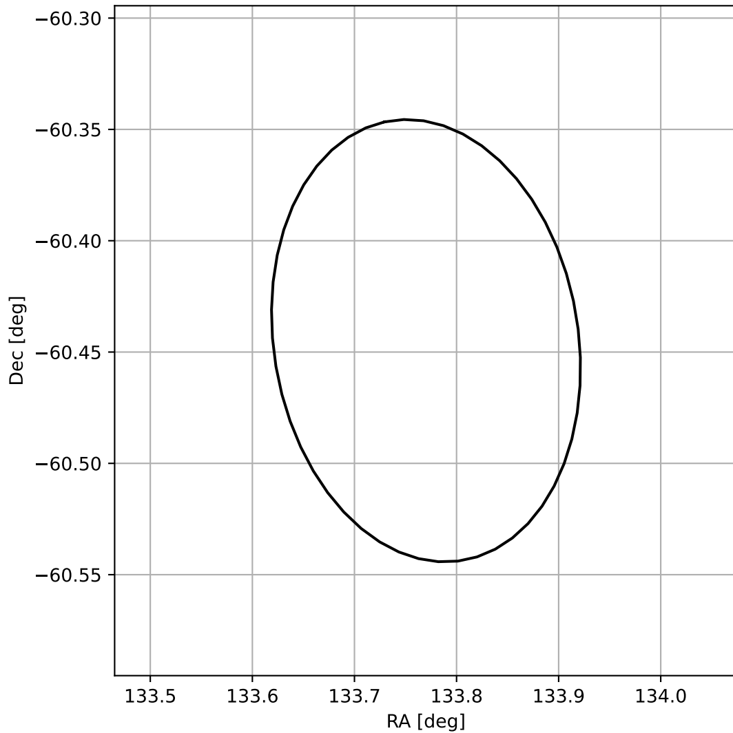
4FGL J0855.0-6026
