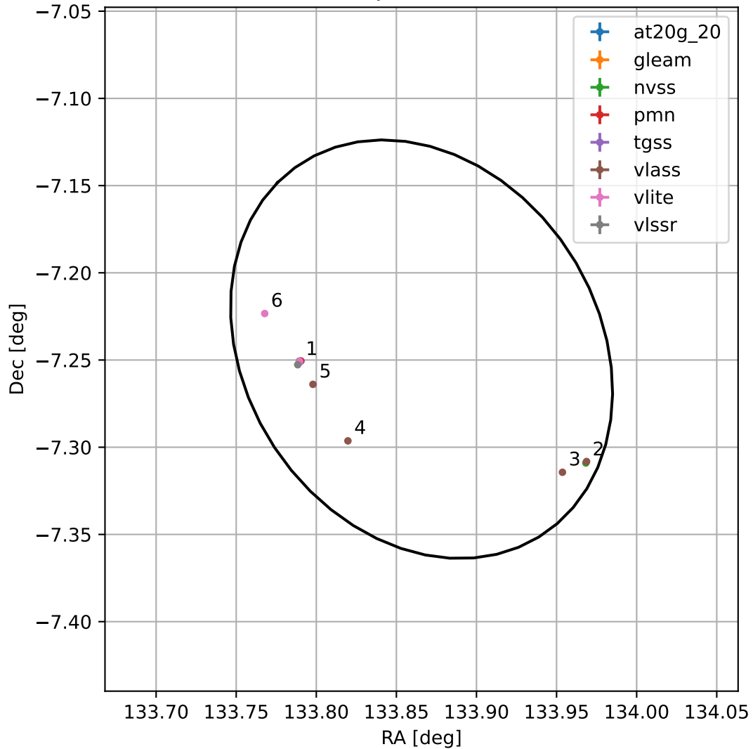
4FGL J0855.4-0714
