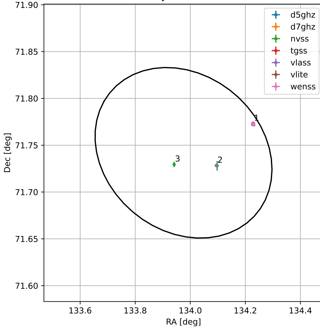
4FGL J0855.9+7144
