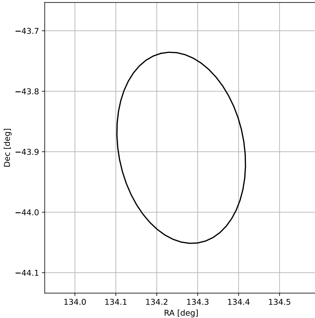
4FGL J0857.0-4353
