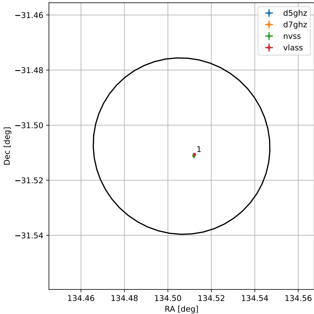
4FGL J0858.0-3130
