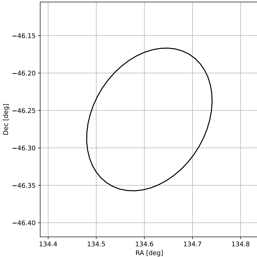
4FGL J0858.4-4615
