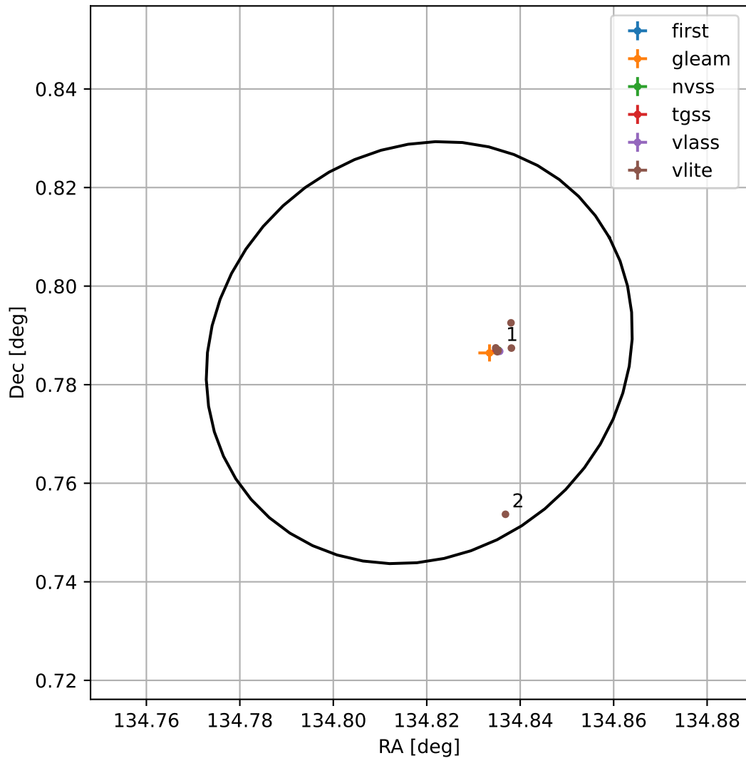
4FGL J0859.2+0047
