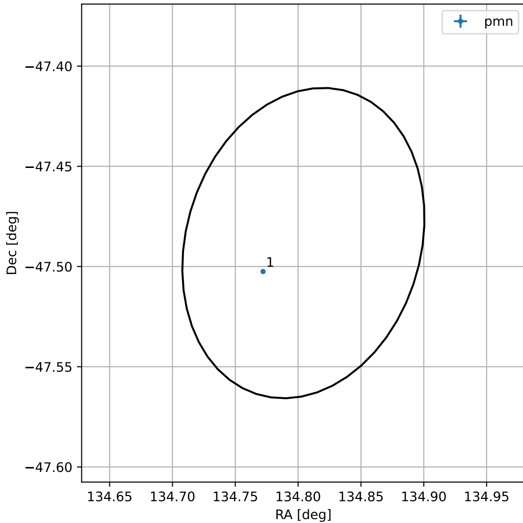
4FGL J0859.2-4729
