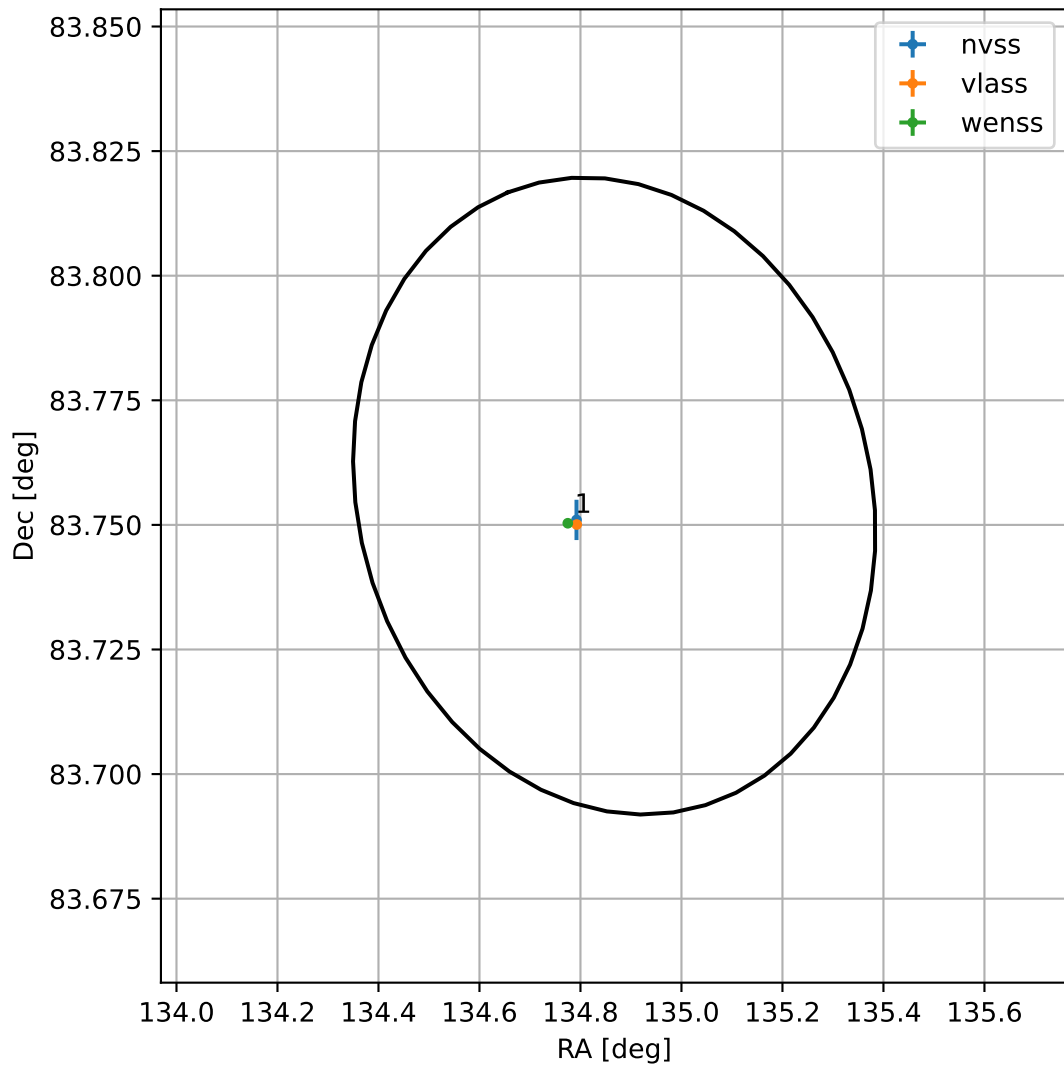
4FGL J0859.4+8345
