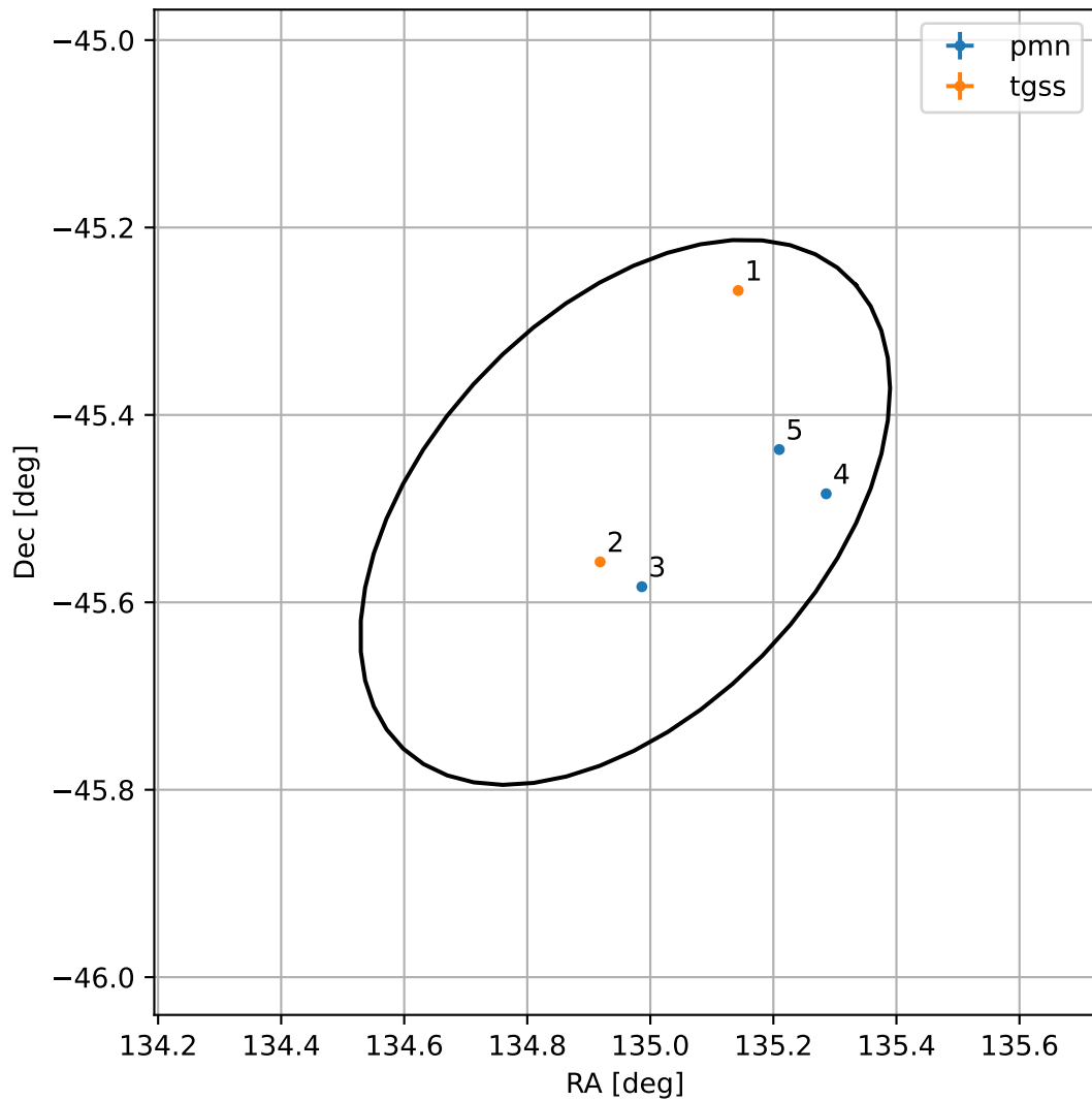
4FGL J0859.8-4530
