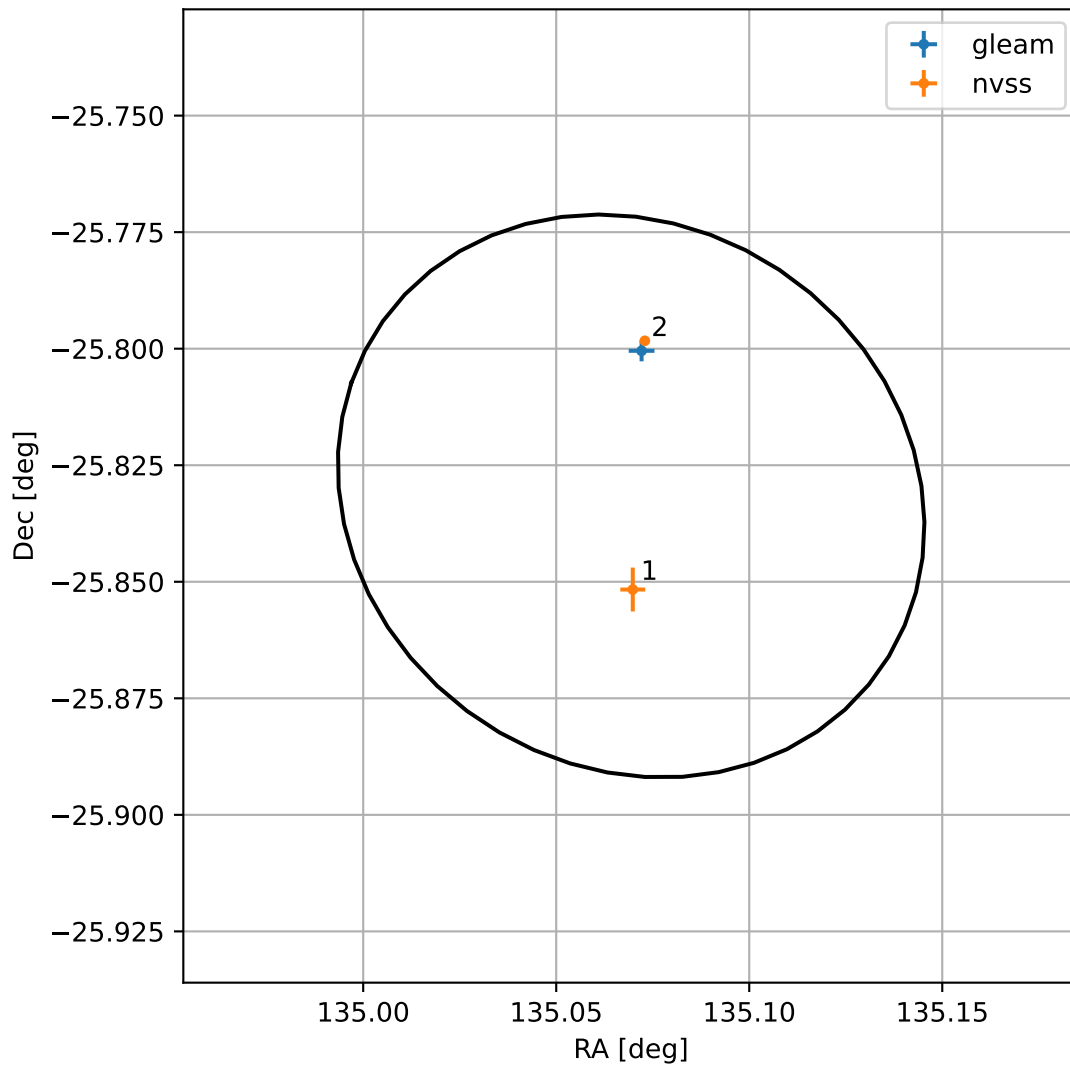
4FGL J0900.2-2549
