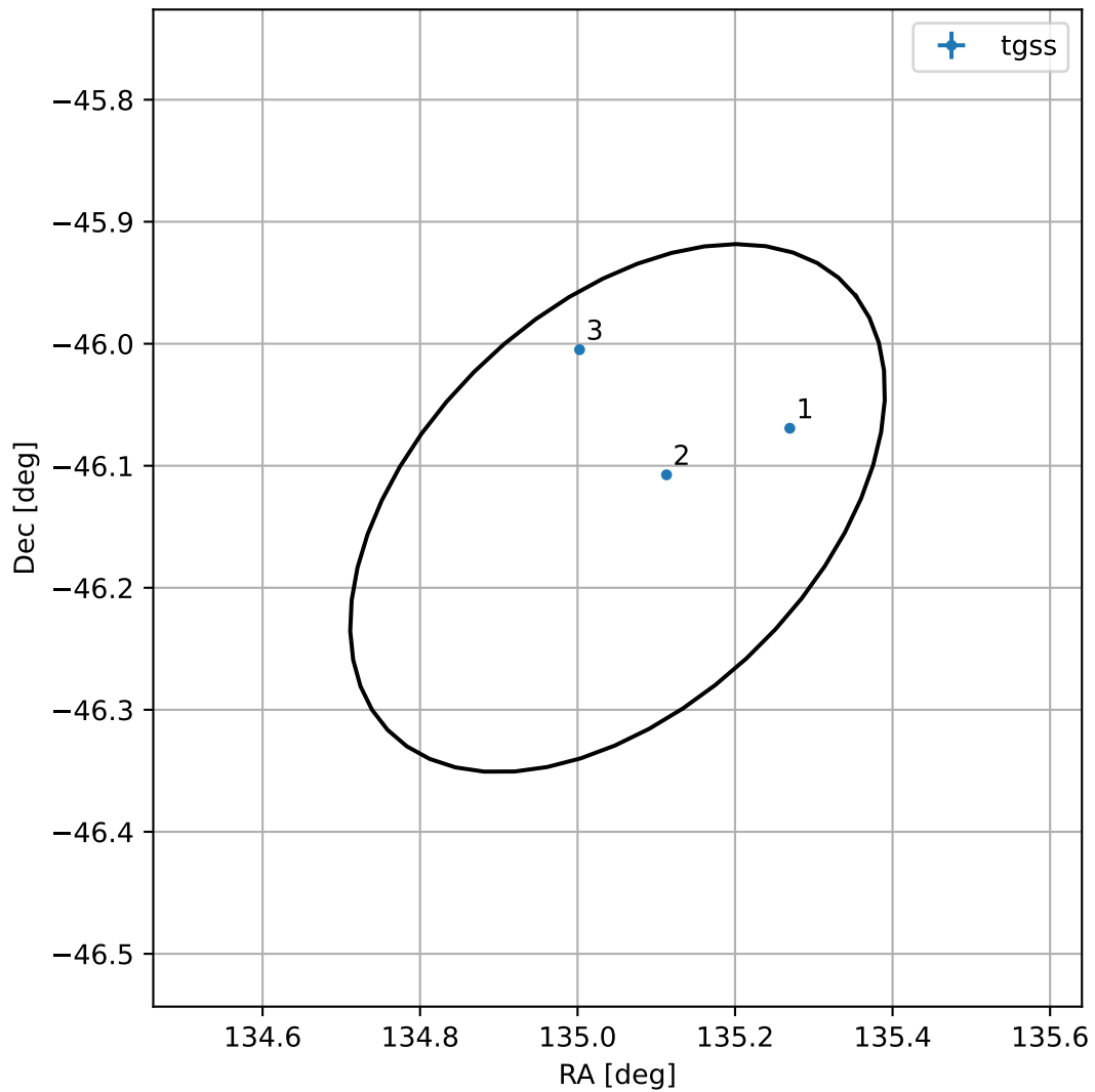
4FGL J0900.2-4608
