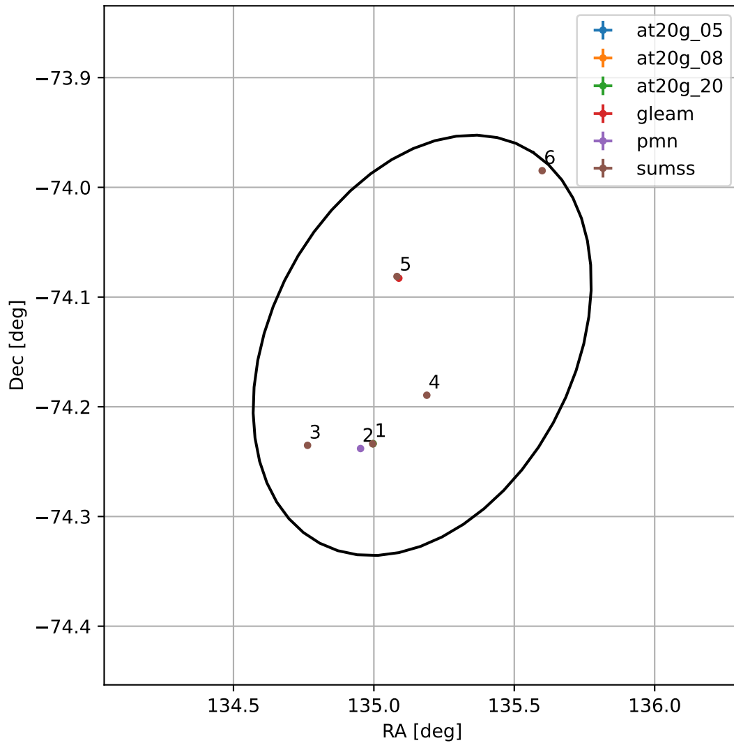
4FGL J0900.6-7408
