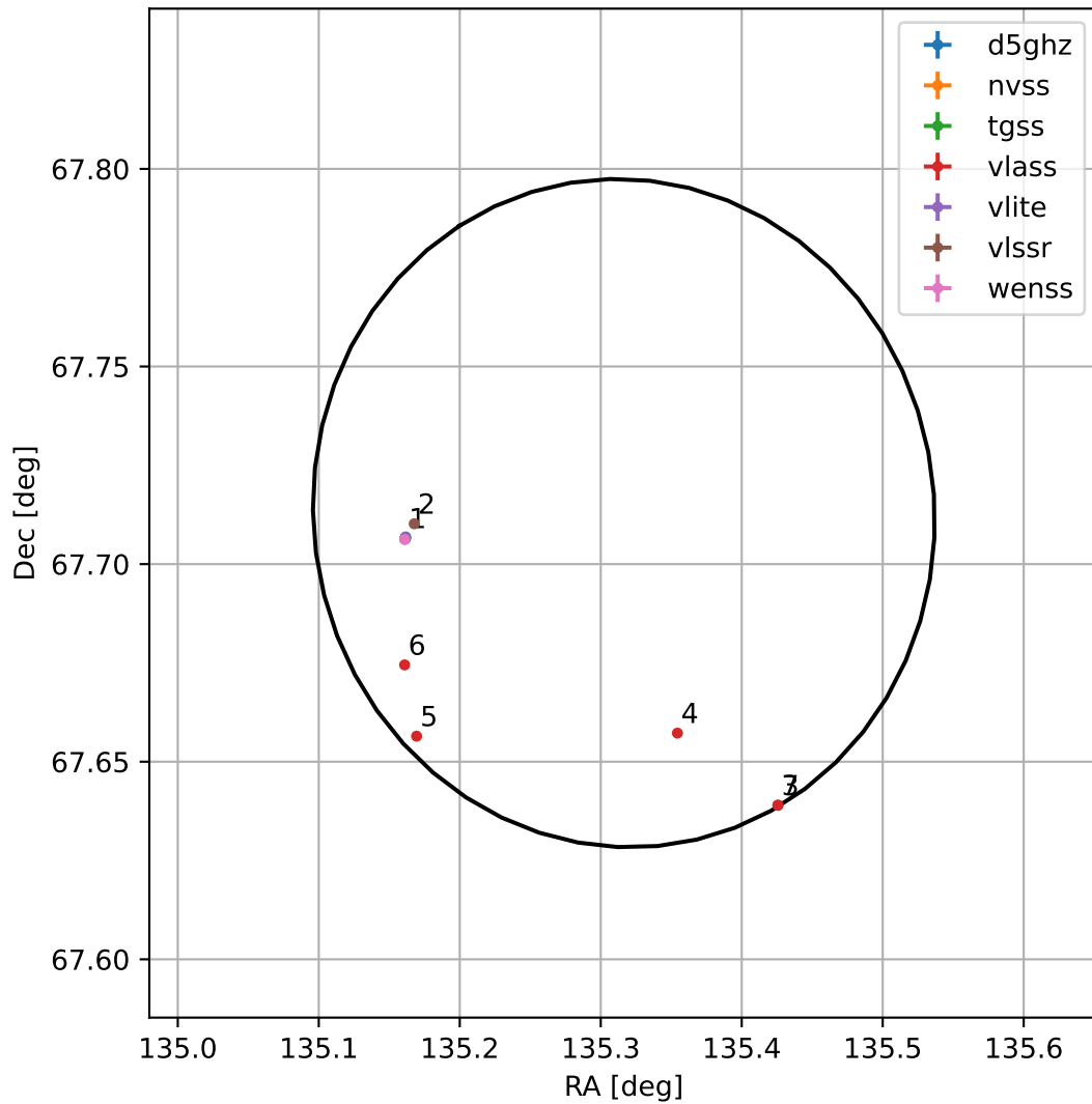
4FGL J0901.2+6742
