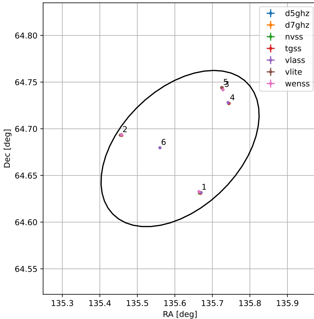
4FGL J0902.4+6440
