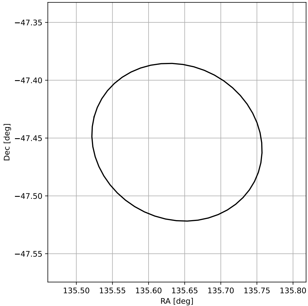
4FGL J0902.5-4727
