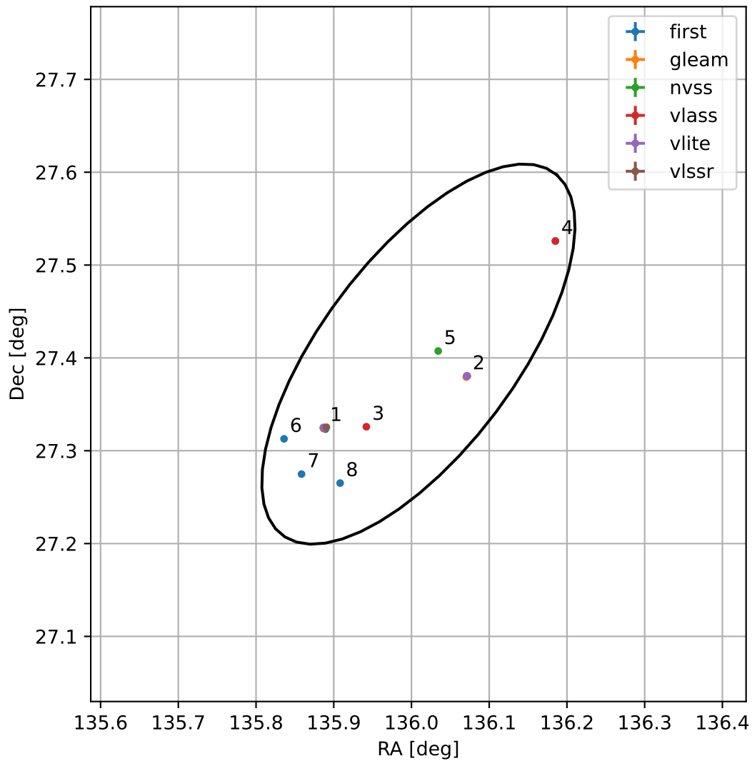
4FGL J0904.0+2724
