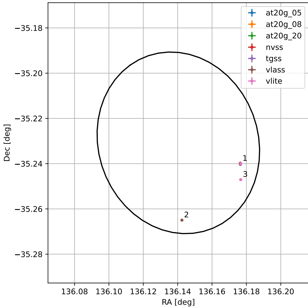
4FGL J0904.5-3513
