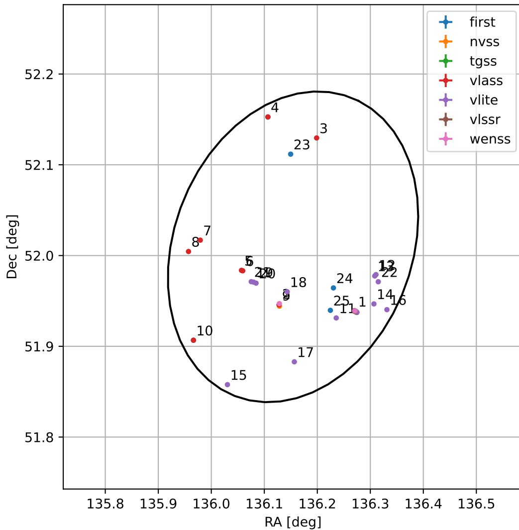
4FGL J0904.6+5200
