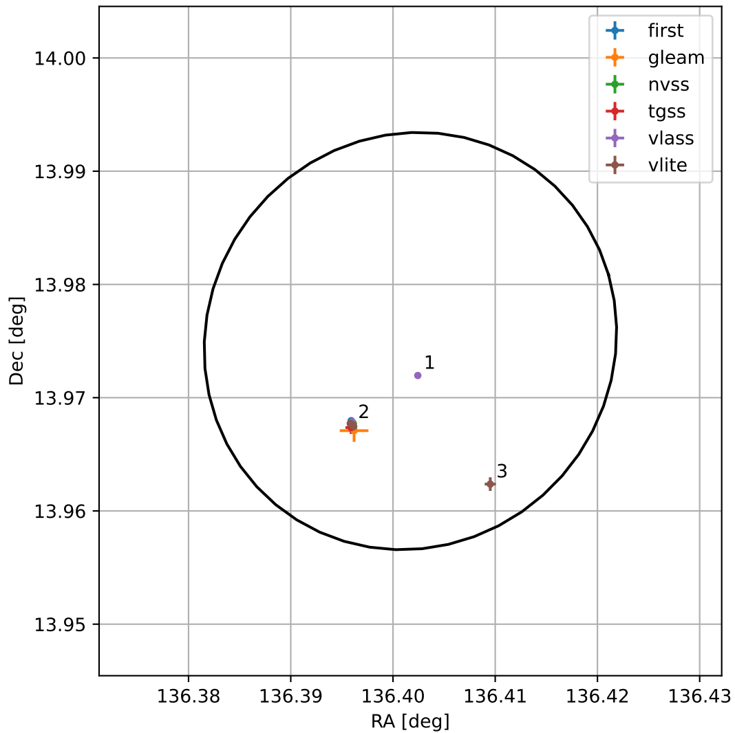
4FGL J0905.6+1358
