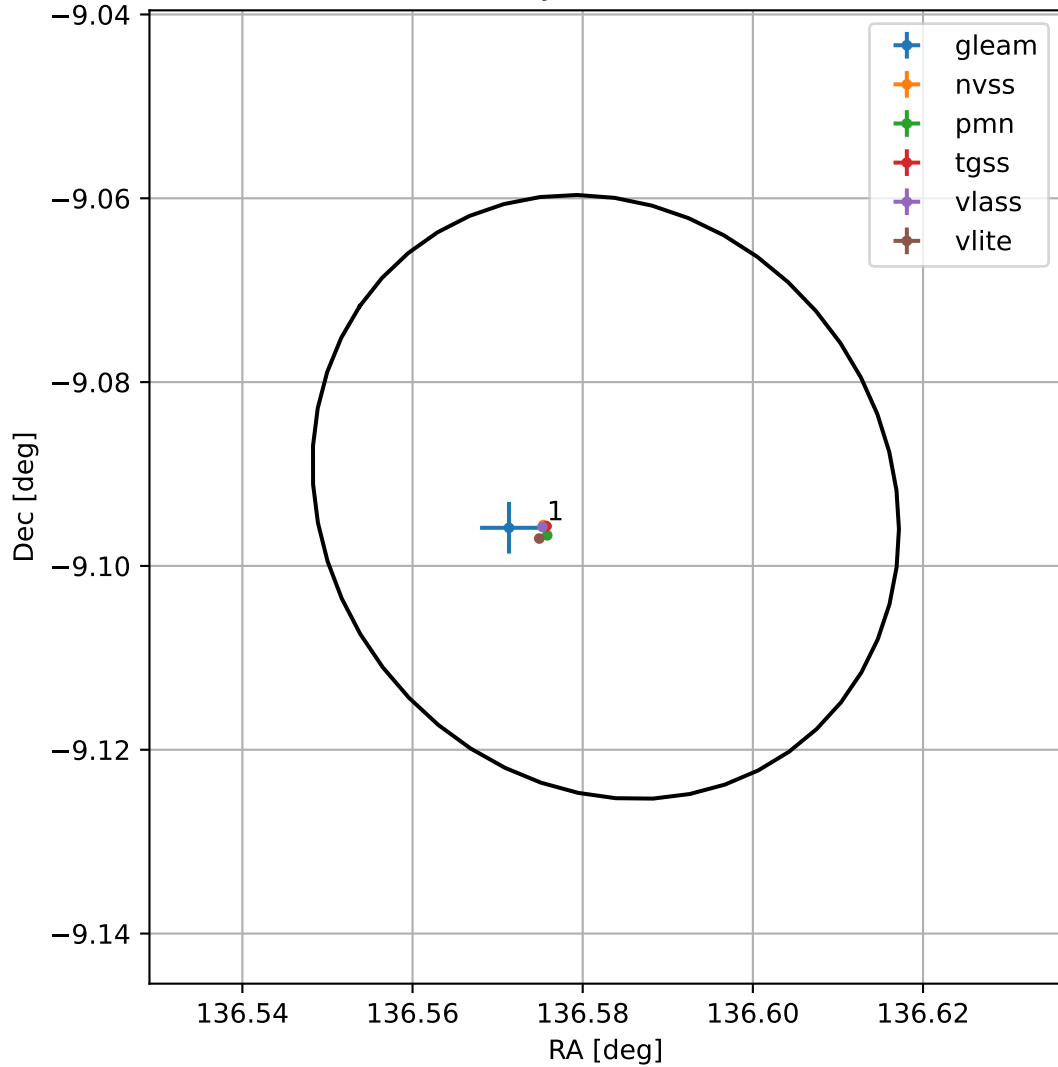
4FGL J0906.3-0905
