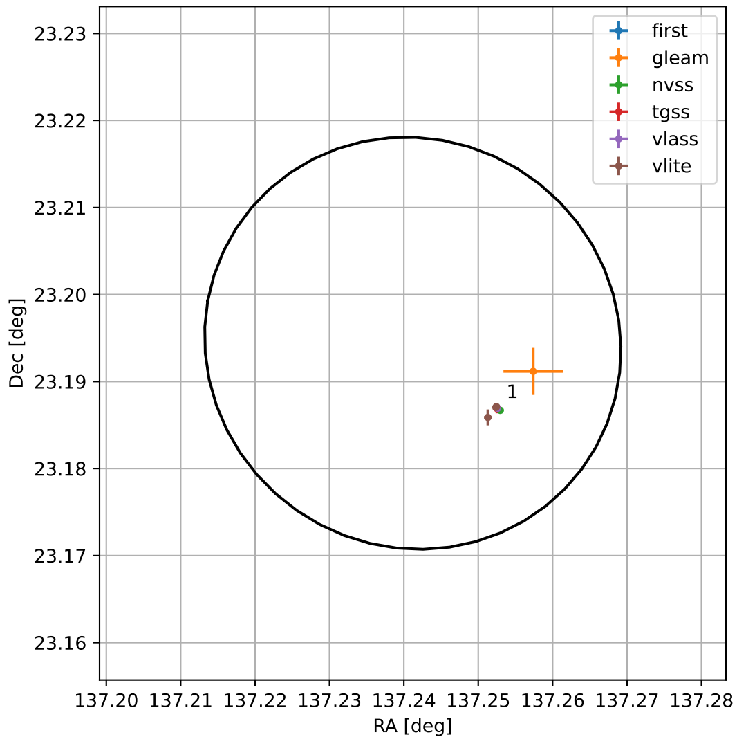
4FGL J0908.9+2311
