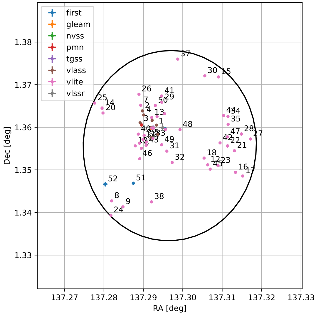
4FGL J0909.1+0121
