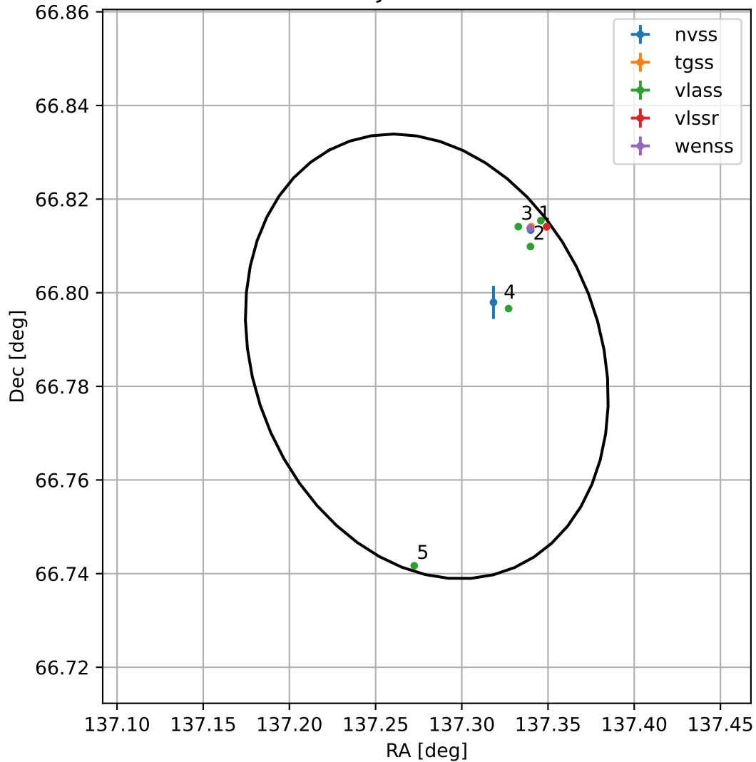
4FGL J0909.1+6647
