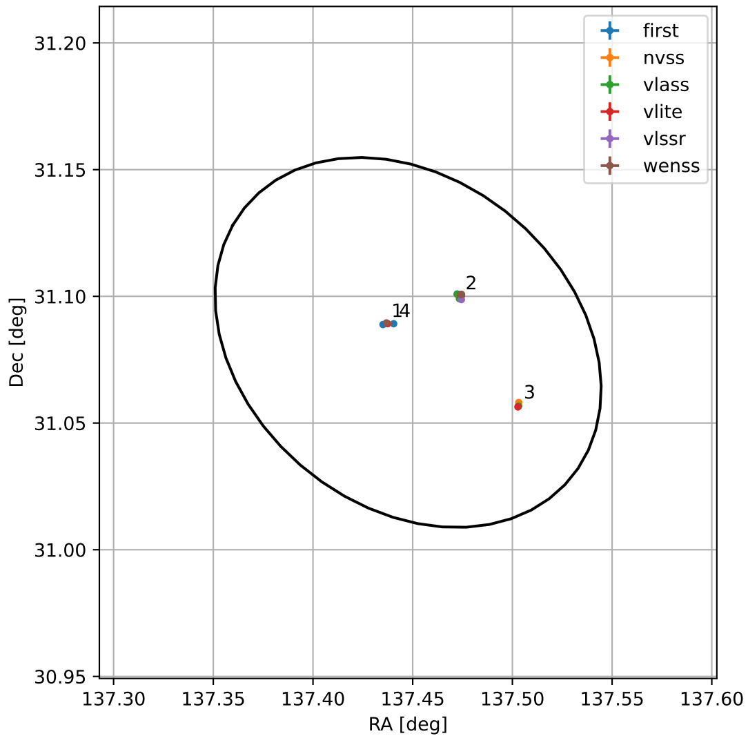
4FGL J0909.7+3104
