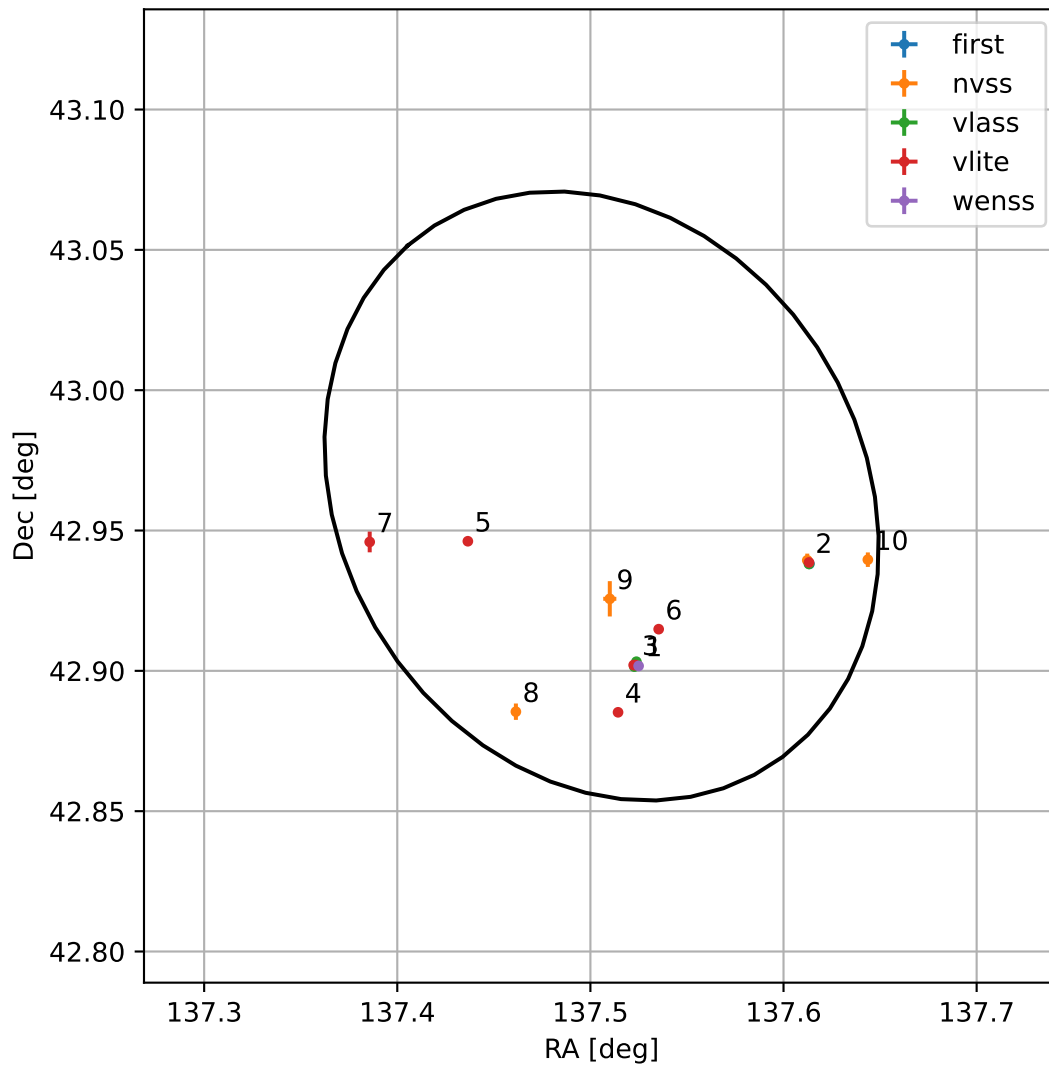
4FGL J0910.0+4257
