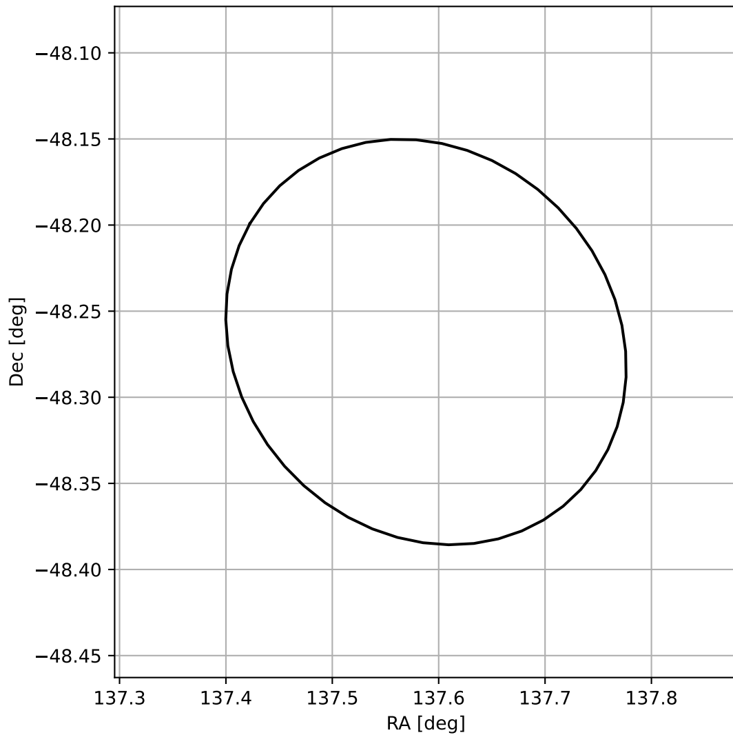
4FGL J0910.3-4816
