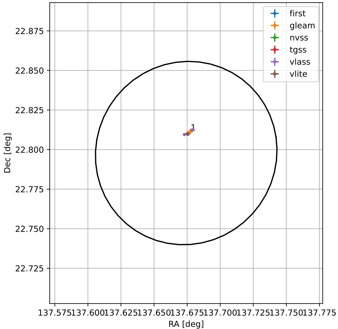
4FGL J0910.6+2247
