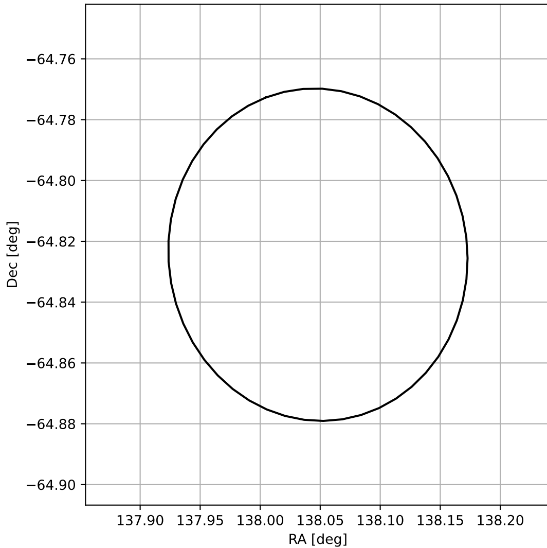
4FGL J0912.1-6449
