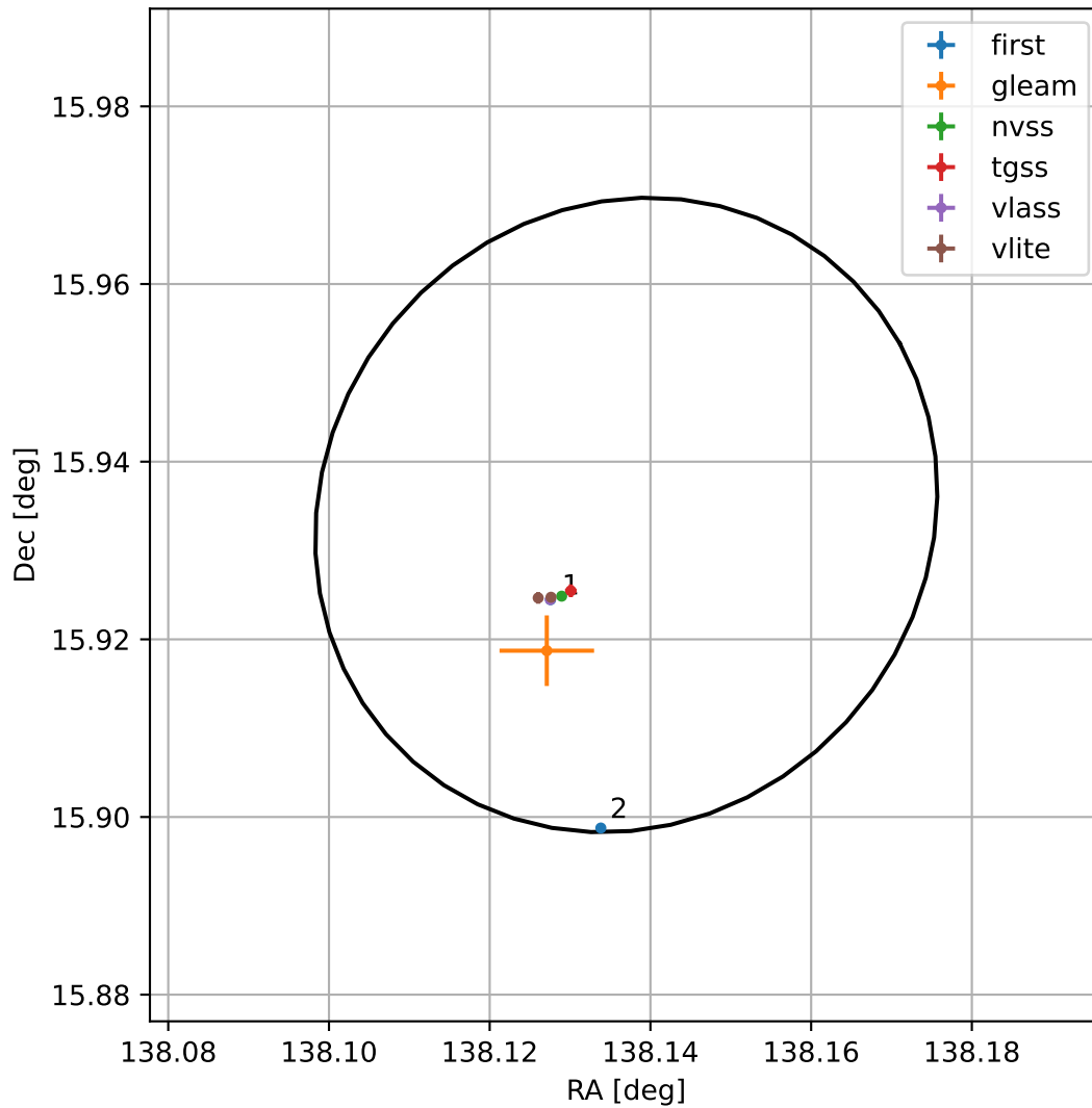
4FGL J0912.5+1556
