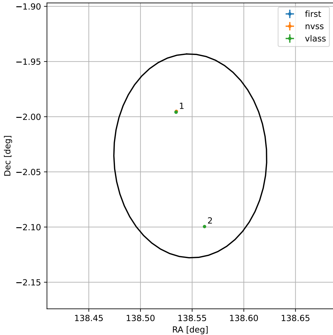
4FGL J0914.1-0202
