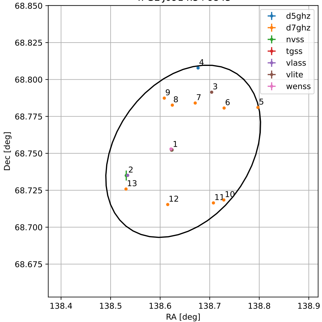
4FGL J0914.5+6845
