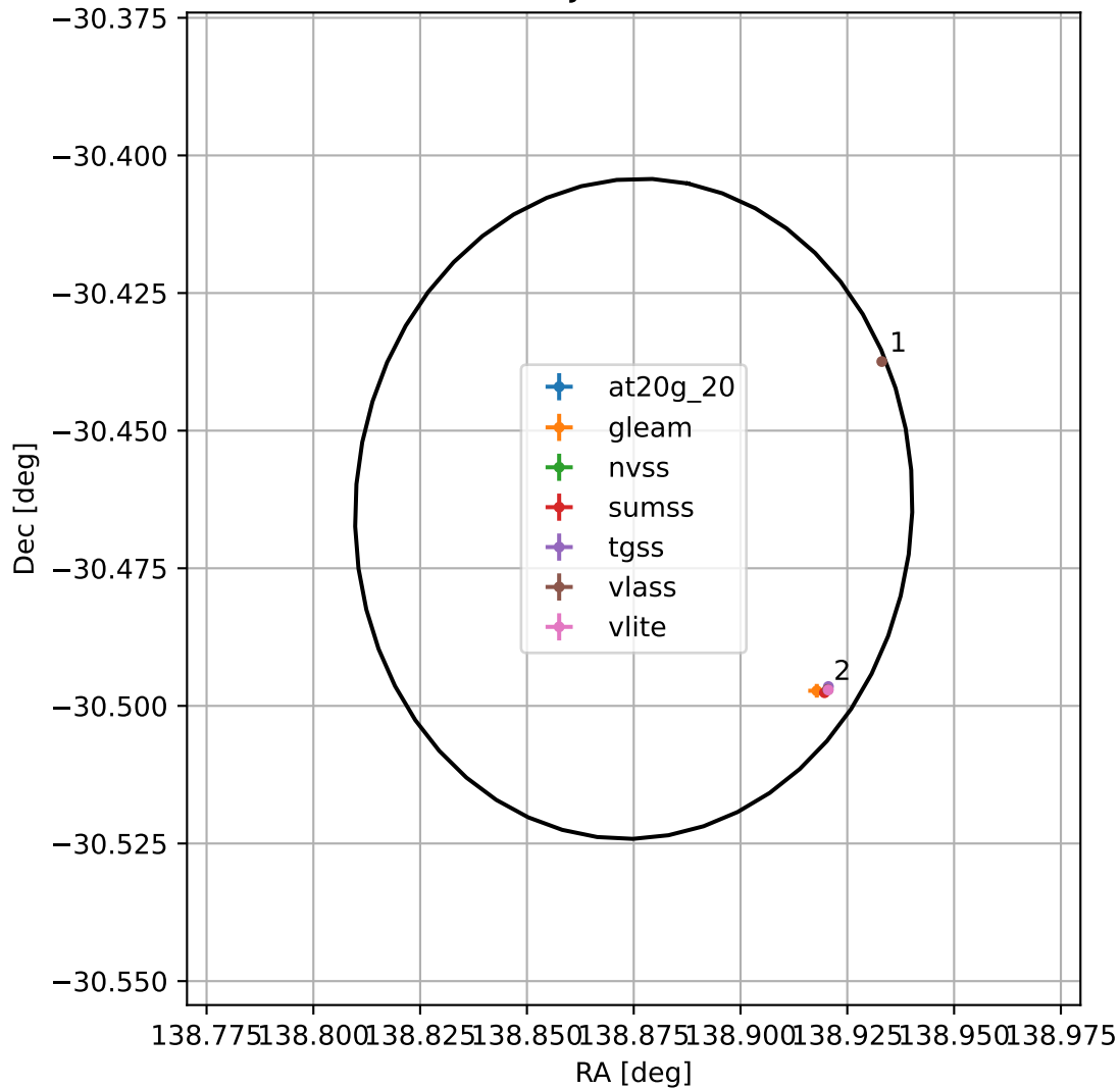
4FGL J0915.4-3027
